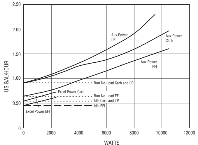
AUXILIARY POWER FUEL CONSUMPTION
