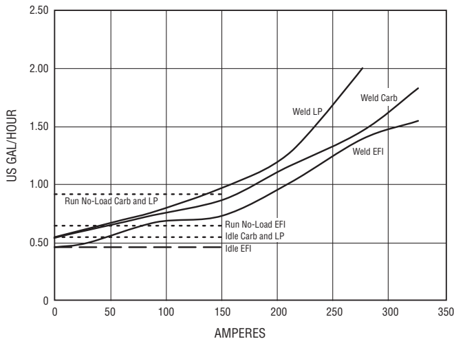
WELD FUEL CONSUMPTION
